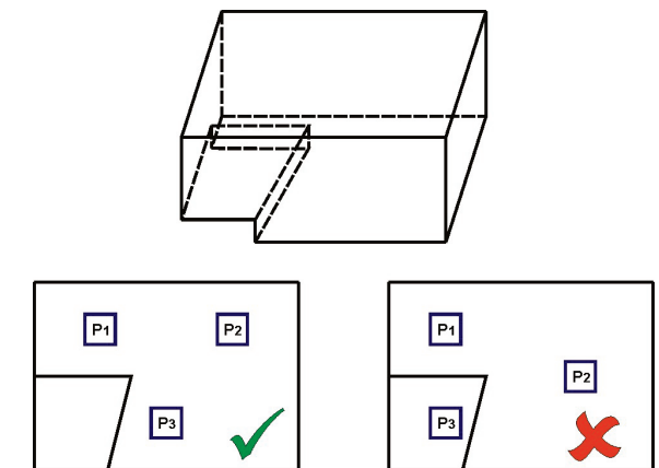
Figure 6 Correct (existent surface) and incorrect (non-existent surface) placement of locating elements
