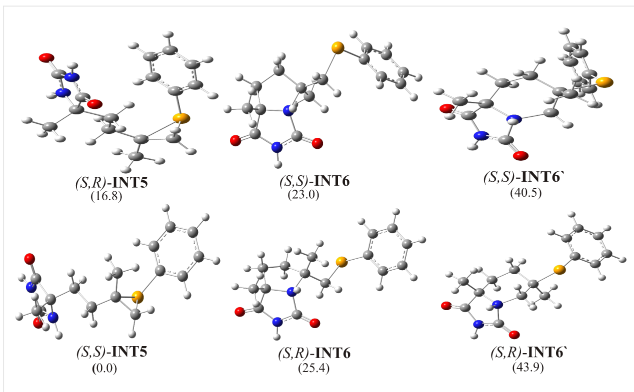
Figure 7: Optimized geometries of possible intermediates of the selenocyclization of model substrate 3 , with relative free energy values indicated in kJ/mol.
