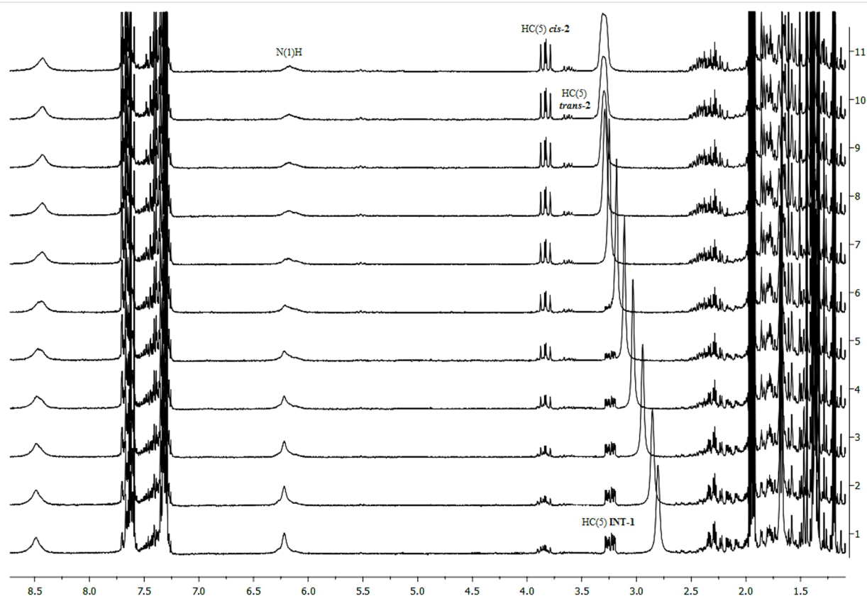
Figure 1: ^1\text{H} NMR monitoring of the cyclization of 5-alkenylhydantoin 1 with PhSeCl in acetonitrile- d_3 solution in the presence of silica gel at ambient temperature during 15 h.
