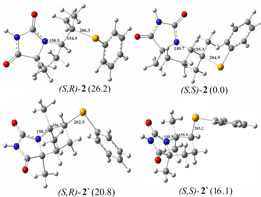
Figure 6: Optimized geometries of possible products of the selenocyclization of 1 , with relative free energy values indicated in kJ/mol. The crucial bond lengths are given in pm.
