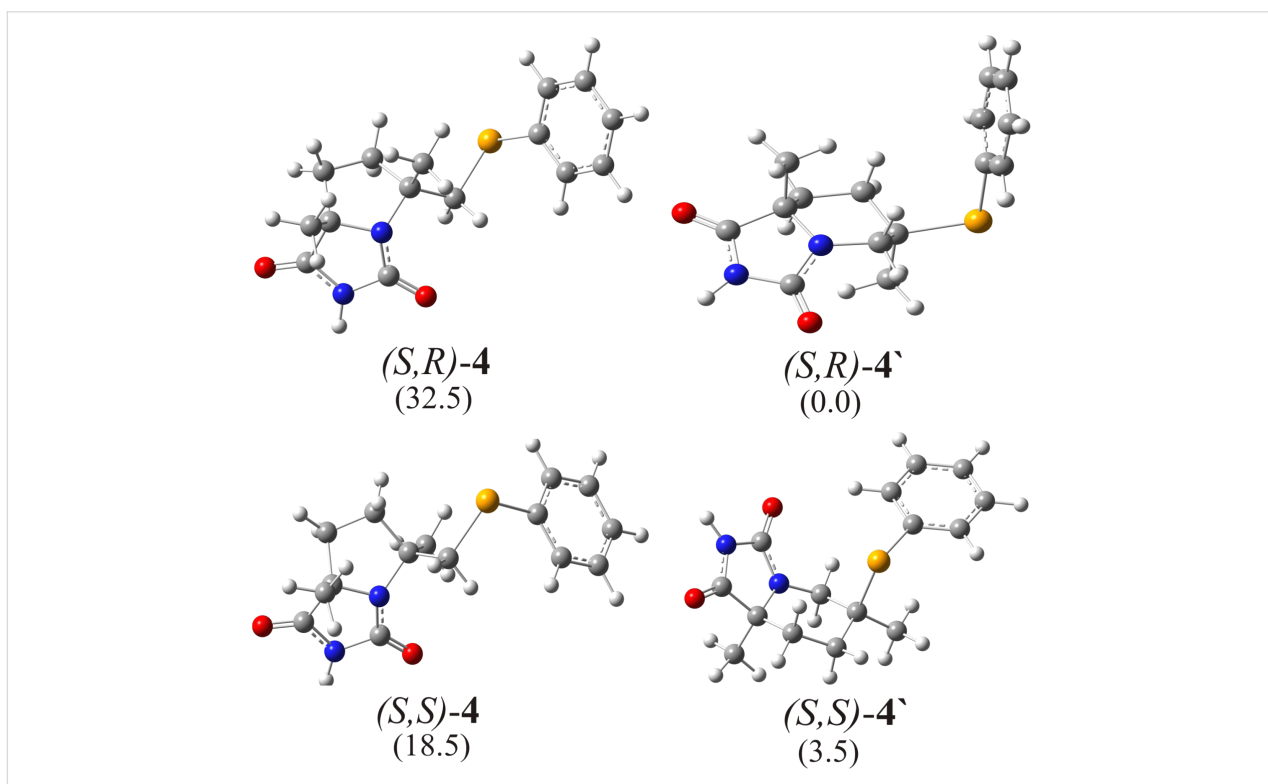
Figure 8: Optimized geometries of possible products of the selenocyclization of model substrate 3 , with relative free energy values indicated in kJ/mol.
