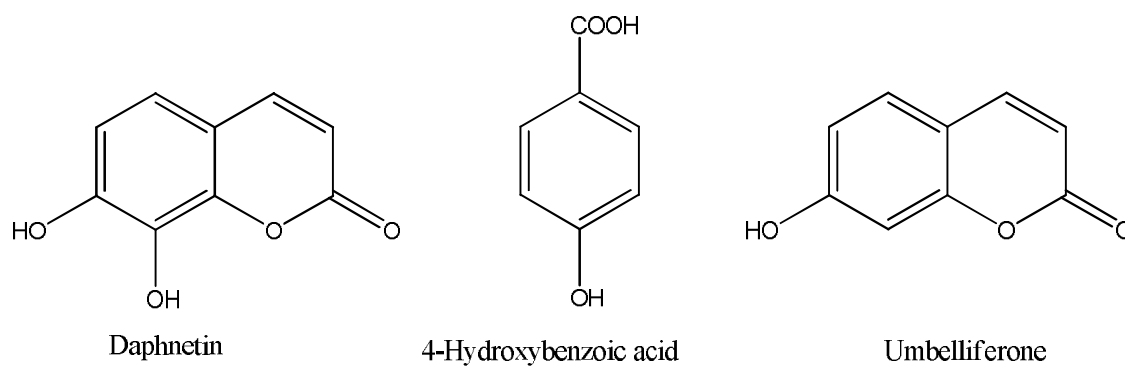
Figure 4: The structures of the identified compounds from HPLC chromatograms of D. alpina extracts
