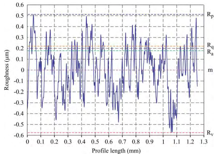
Figure 14: Diagram of measured roughness profile.
