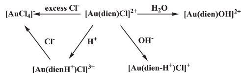
Scheme 2 Influence of the reaction conditions on the formation of different reaction species of the [\text{Au}(\text{dien})\text{Cl}]^{2+} complex.
