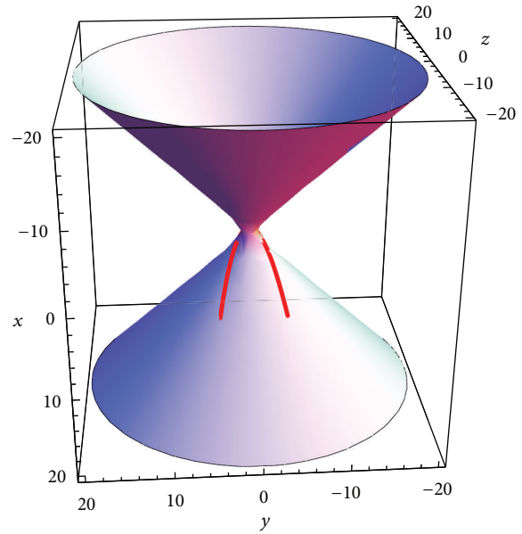
FIGURE 1: The curve \alpha on S_1^2 .
