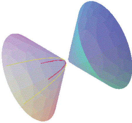
FIGURE 2: The \alpha\xi -pseudohyperbolic Smarandache curve \beta and the curve \alpha on H_0^2(1) .
