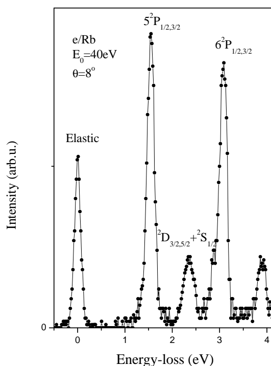
Figure 1. Energy-loss spectrum of rubidium.
