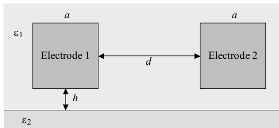
Fig. 19. Two wire line above infinite dielectric surface
