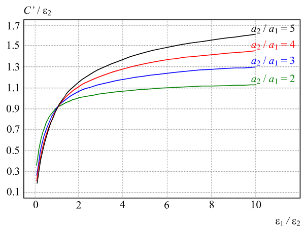
Fig. 18. The ratio C'/\varepsilon_2 for different ratios a_1/a_2 and \varepsilon_1/\varepsilon_2 , when d_1/a_1 = 18
