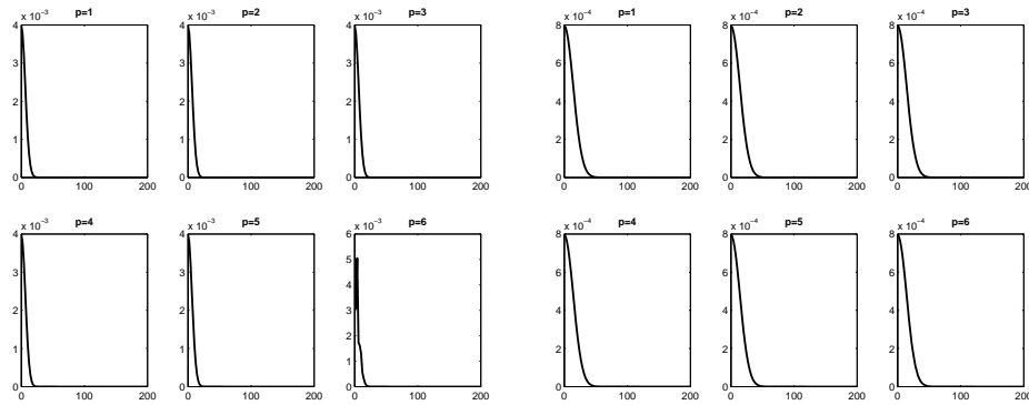
Fig. 1 2D heat, BDF: \omega_{20}(1; d) (left-side) and \omega_{100}(1; d) (right-side), d = 0.01 : 200 .
